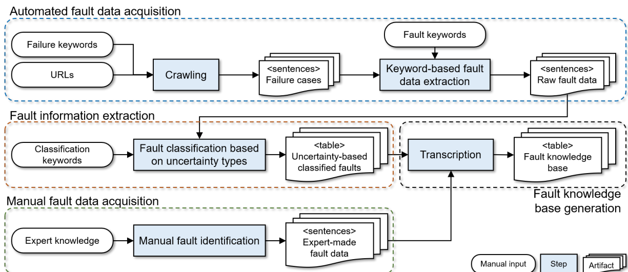
Fig. 1: Approach overview
